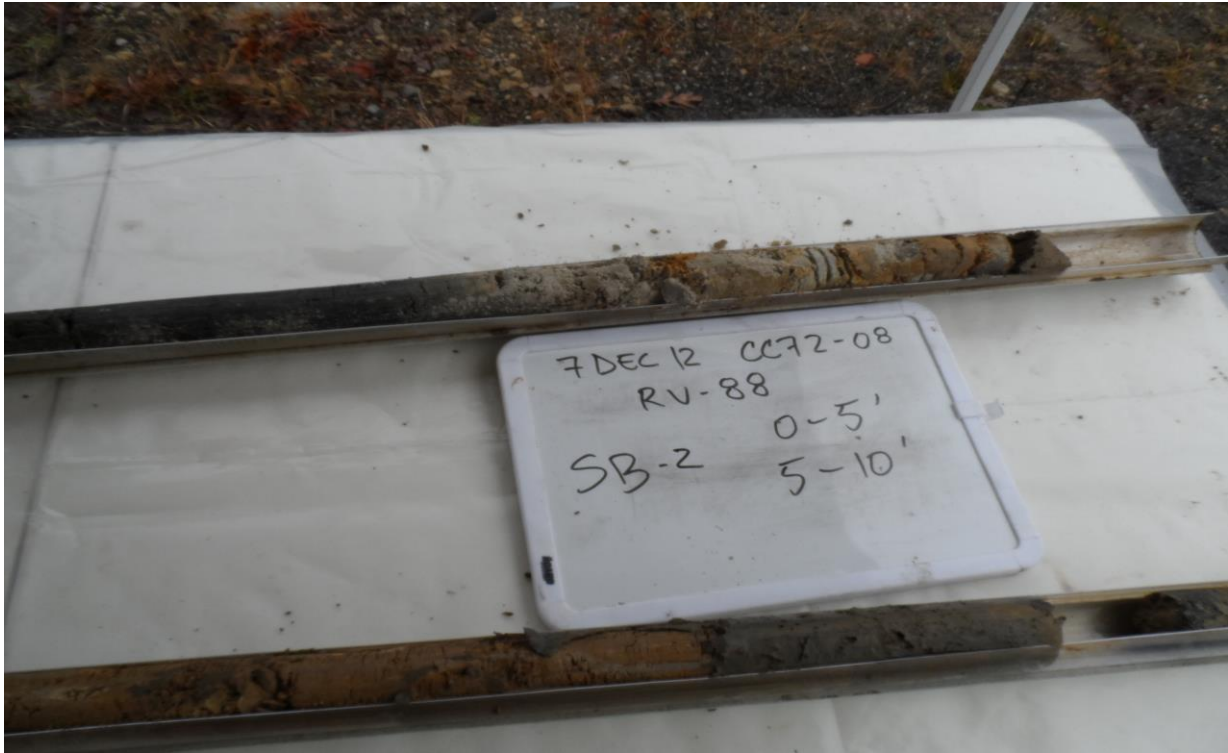
View of soil sampling intervals 0-5 and 5-10 ft, at boring SB02 at former UST RV-88.
