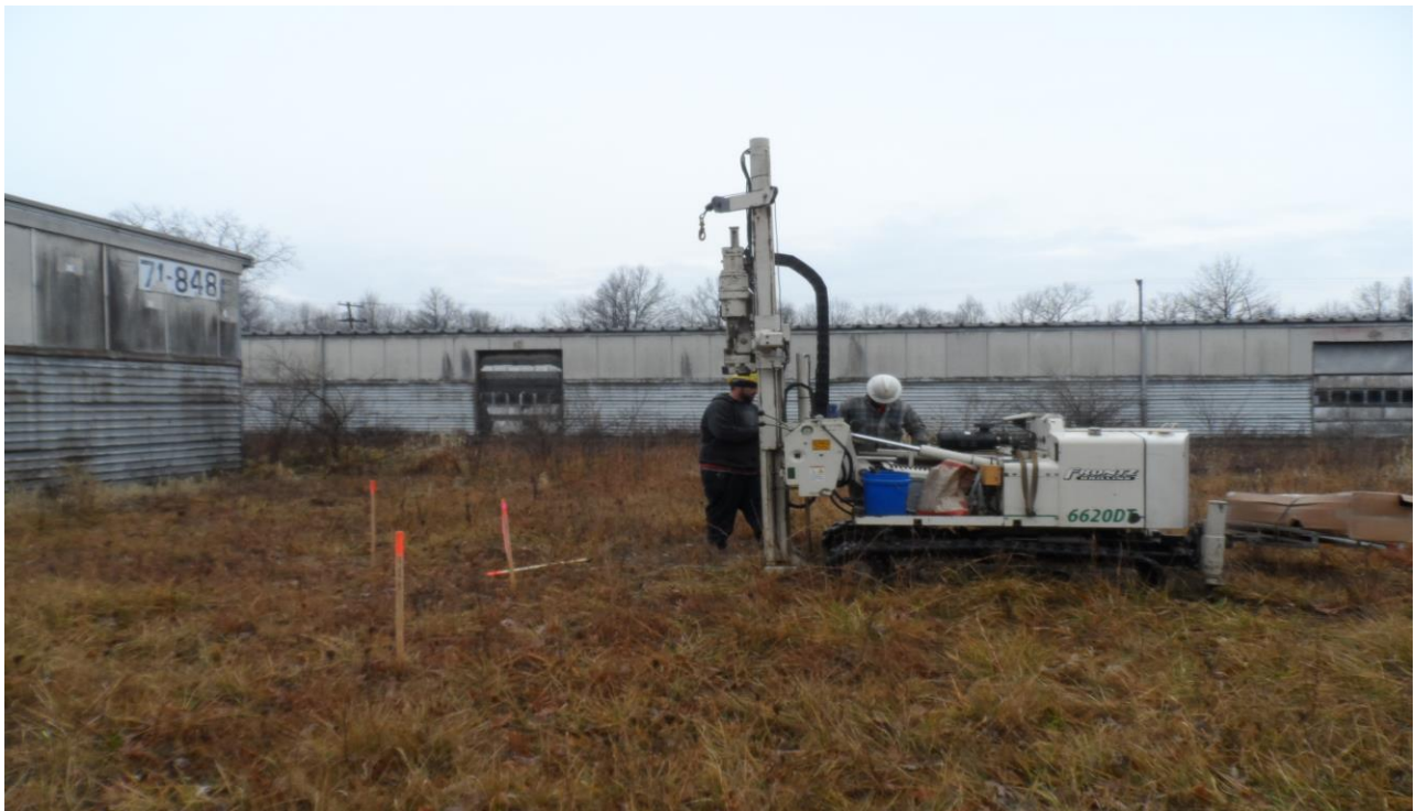
View of direct-push drilling activities at former UST location CC-RVAAP-72-08 at Building 71-848.
